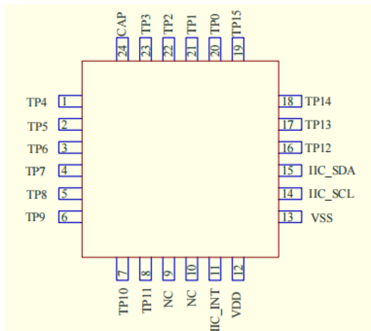
QFN24
